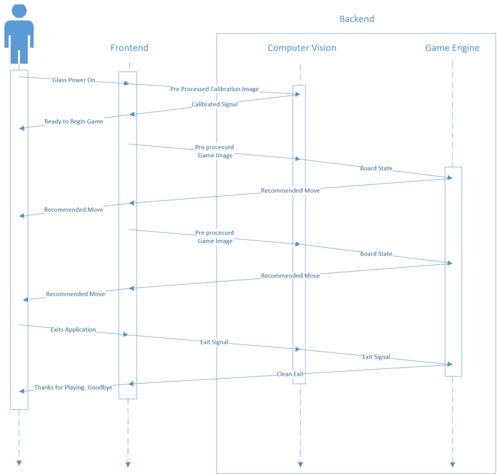
Figure 6: High Level Sequence Diagram
